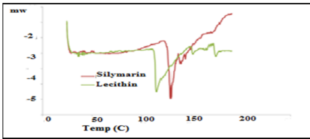
Figure 4: DSC graph of silymarin and lecithin
