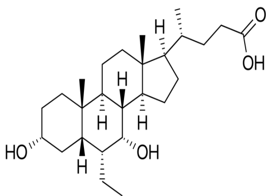
Figure 1: Chemical Structure of Obeticholic acid.
