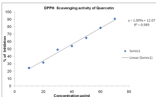
Figure 3: Results of DPPH radical scavenging assay of Quercetin
