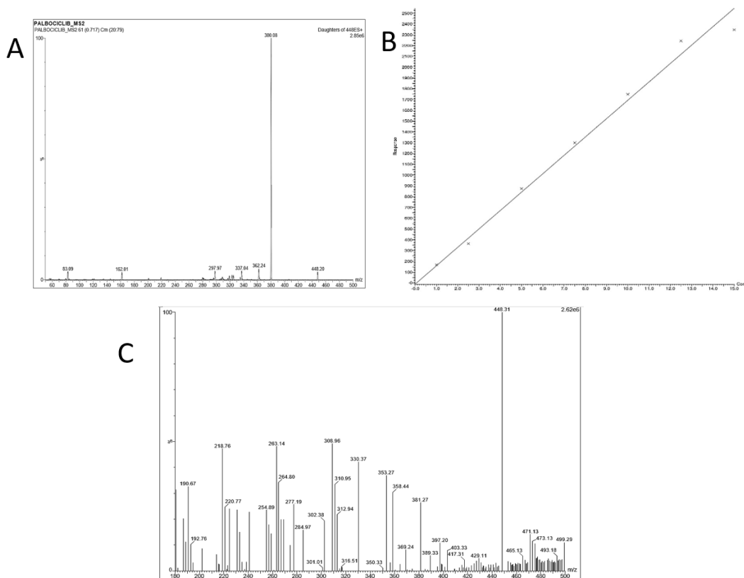
Figure 3: A) Mass spectra depicting Palbociclib API with m/z value of 448.20 with a base peak at m/z 380.08. B) Mass spectra depicting PCB in capsule formulation with m/z value of 448.31. C) Graph illustrating linearity results of Palbociclib in bulk drug.
