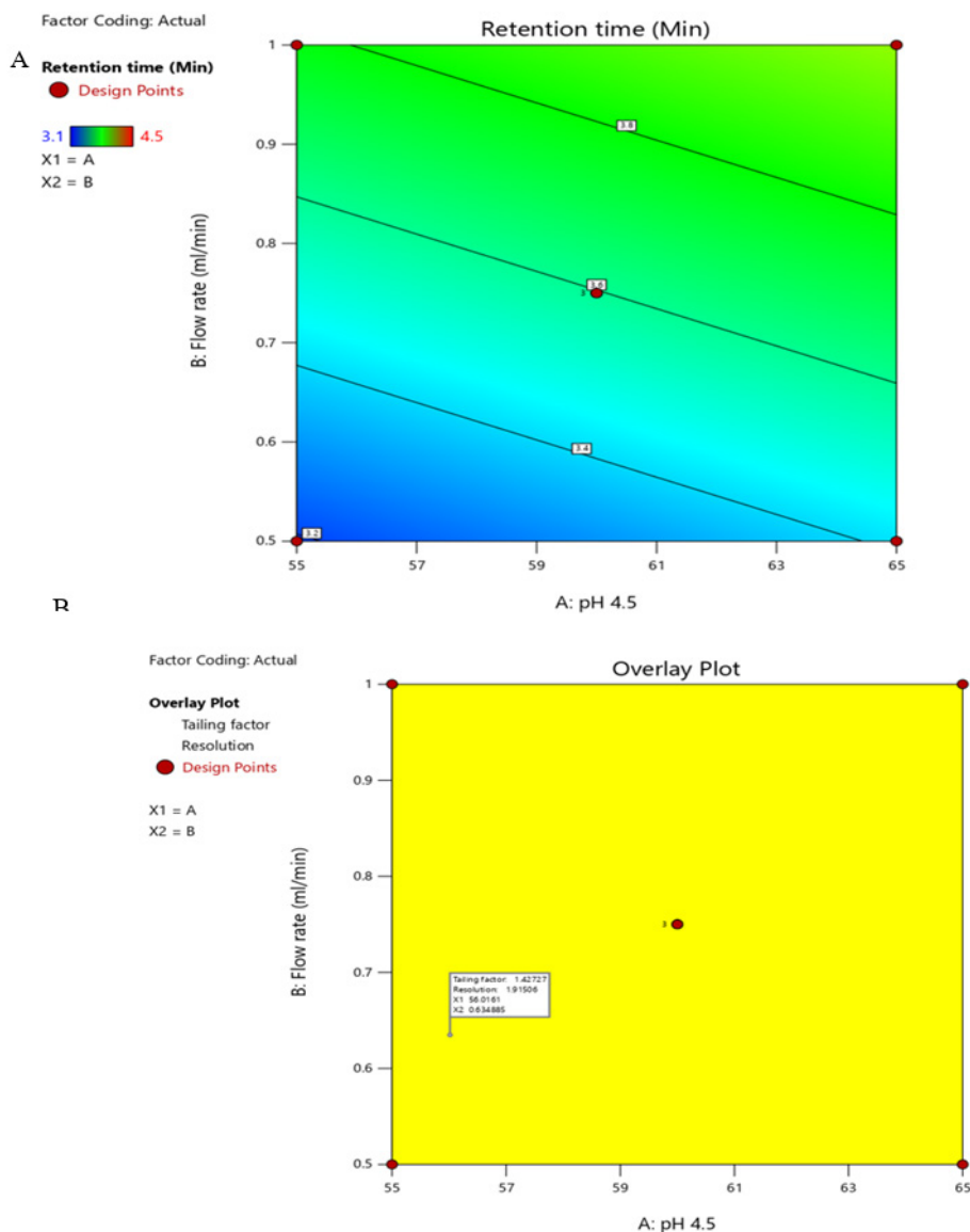
Figure 2: Graph representing A) Effect of variables x1 and x2 on retention time. B) overlay of x1 and x2 on tailing factor along with resolution.
