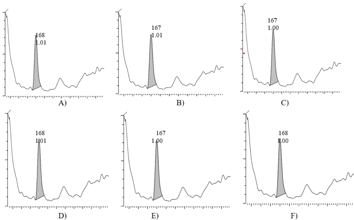
Figure 4: A) LC obtained Chromatograms showing Intraday precision at LOQ Level A-F: Injections (1-6) B) LC obtained chromatograms (A-C) showing injections (1-3) in triplicate of PCB at spiked 50% of Drug product concentration. C) LC obtained chromatograms showing injections in triplicate of PCB at spiked 100% of Drug product concentration. D) LC obtained chromatograms (A-C) showing injections in triplicate of PCB at spiked 150% of Drug product concentration.
