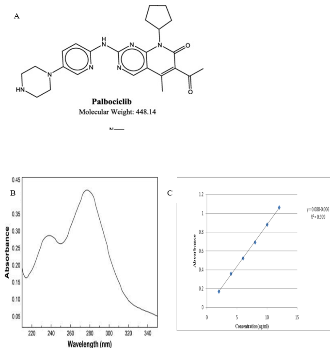
Figure 1: A) Structure of Palbociclib B) UV-vis Spectrum showing Palbociclib in methanol C) Calibration Curve of Palbociclib at 220 nm.
