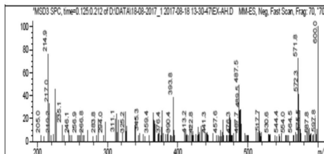
Figure 12: LCMS Data of isolate from AF.
