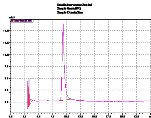
Figure 4: (d) Chromatogram of Buparvaquone after oxidative degradation.
