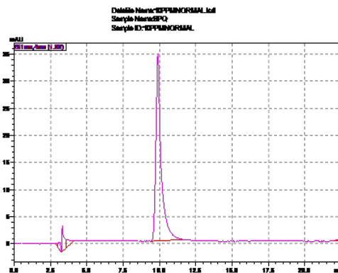
Figure 4: (e) Chromatogram of Buparvaquone after thermal degradation.
