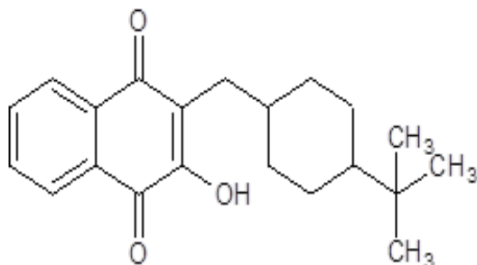
Figure 1: Structure of Buparvaquone.
