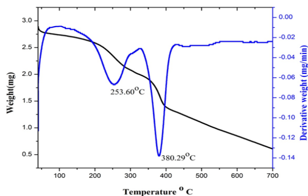
Figure S1: 3a: Thermogram of Co(II) complex 5.
