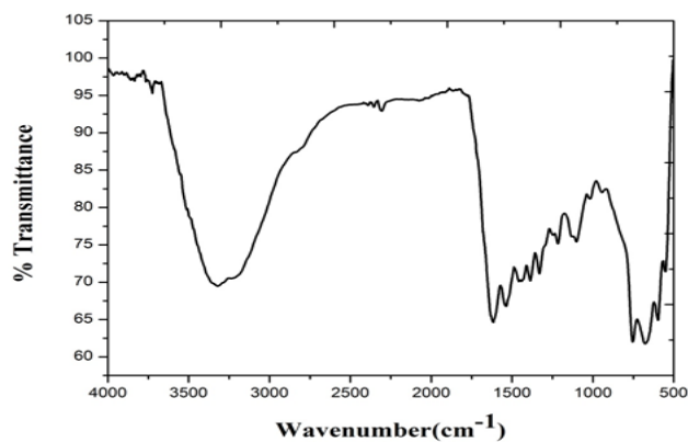
Figure S1: 2f: FT-IR spectrum of Co(II) complex 6.
