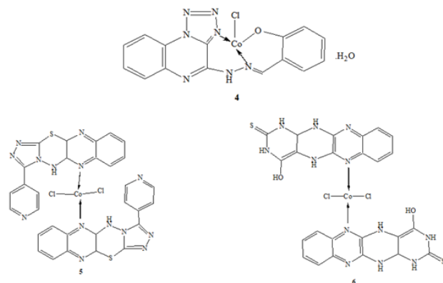
Figure 2A: Proposed geometry of the complexes.
