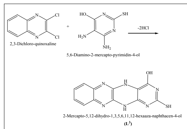
Scheme 3: Synthesis of ligand 3 ( L^3 ).
