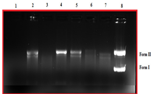
Figure 4: Changes in the agarose gel electrophoretic pattern of pBr322 DNA induced by H_2O_2 and Co(III) complexes, lane 1, DNA alone; lane 2, DNA + H_2O_2 ; lane 3, DNA(20 \mu M) +4 H_2O_2 ; lane 4, DNA(40 \mu M) +4 H_2O_2 ; lane 5, DNA(20 \mu M)+5 H_2O_2 ; lane 6, DNA(40 \mu M) +5 H_2O_2 ; lane 7, DNA(20 \mu M) +6 H_2O_2 , lane 8, DNA(40 \mu M) +6 H_2O_2 .
