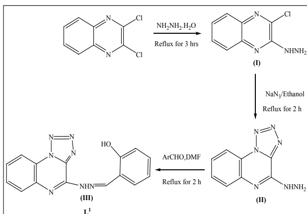
Scheme 1: Synthesis of ligand 1 ( L^1 ).
