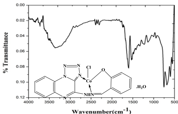
Figure S1: 2d: FT-IR spectrum of Co(II) complex 4.
