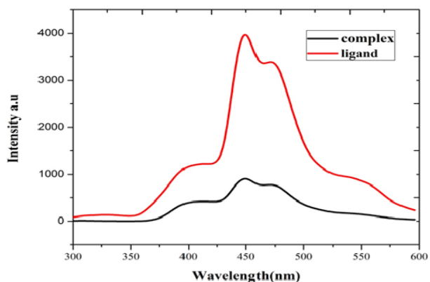
Figure 3B: Fluorescence spectra of the ligand L 2 and its Co(II) complex 5.
