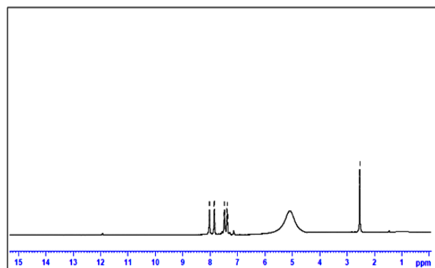
Figure S1: 1b: ^1H -NMR spectrum of Ligand 2 ( L^2 ).
