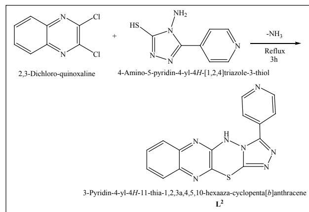
Scheme 2: Synthesis of ligand 2 ( L^2 ).
