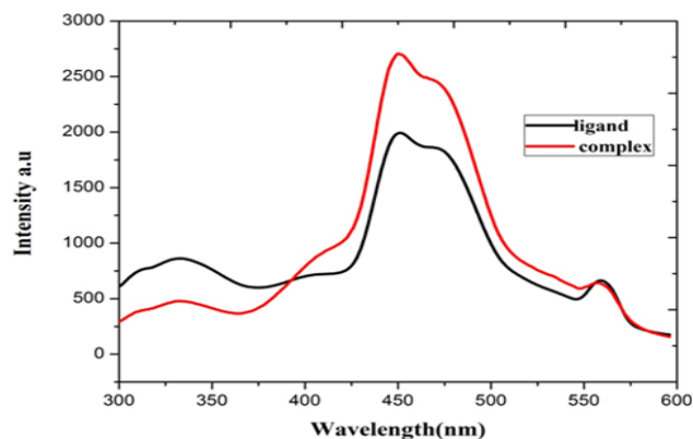
Figure 3C: Fluorescence spectra of the ligand L 3 and its Co(II) complex 6.
