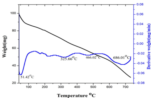
Figure 2: Thermogram of Co(II) complex 4.
