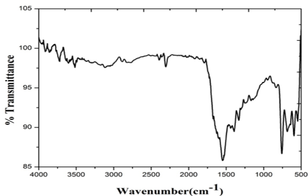
Figure S1: 2c: FT-IR spectrum of ligand 3 (L 3 ).
