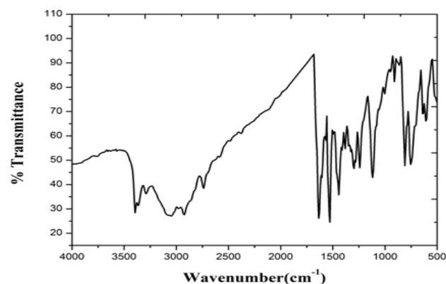
Figure S1: 2b: FT-IR spectrum of ligand 2 ( L^2 ).
