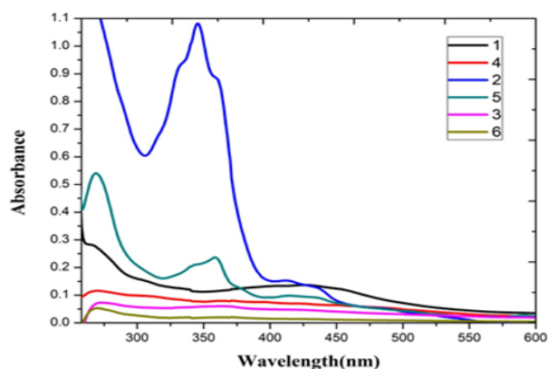
Figure 1: Electronic spectrum of the complexes.
