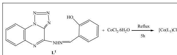
Scheme S1: 1a: Synthesis of Co(II) complex 4.
