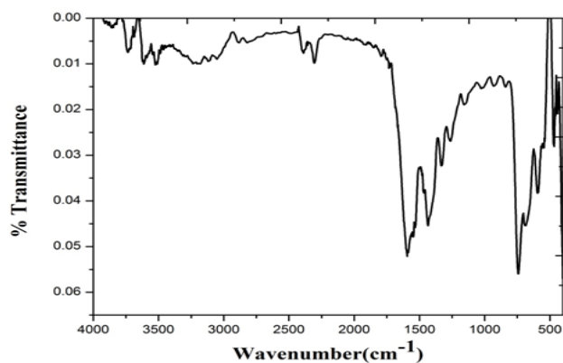
Figure S1: 2a: FT-IR spectrum of ligand 1 ( L^1 ).
