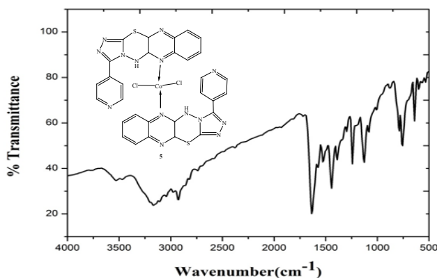
Figure S1: 2e: FT-IR spectrum of Co(II) complex 5.
