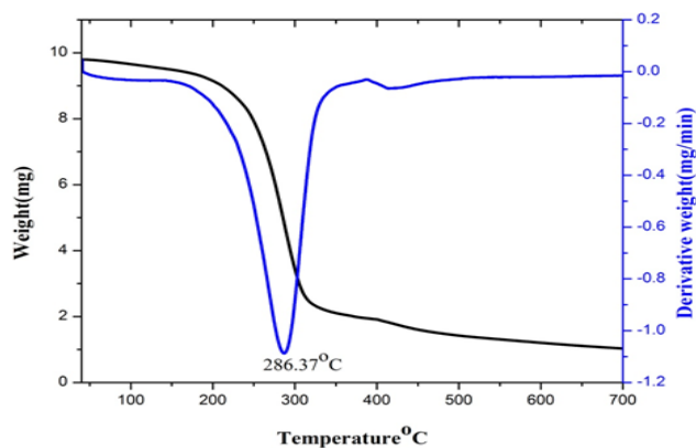
Figure S1: 3b: Thermogram of Co(II) complex 6.
