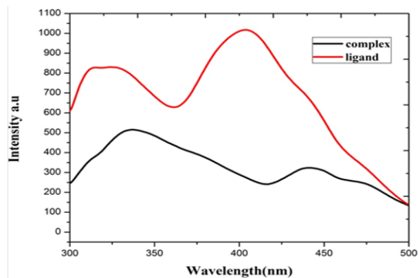
Figure 3A: Fluorescence spectra of the ligand L 1 and its Co(II) complex 4.
