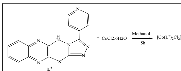
Scheme S1: 1b: Synthesis of Co(II) complex 5.
