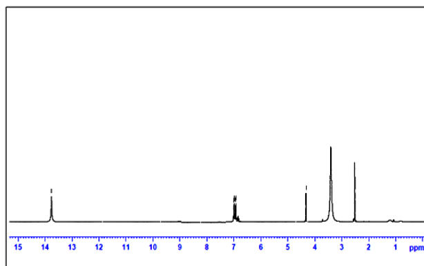
Figure S1: 1c: ^1H -NMR spectrum of Ligand 3 ( L^3 ).
