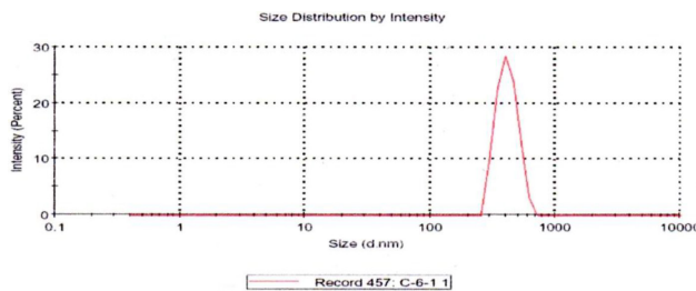
Figure 8: Particle size Copper nanoparticle.
