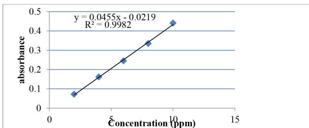
Figure 5: Standard calibration curve for different dilution of mupirocin at 220 nm.
