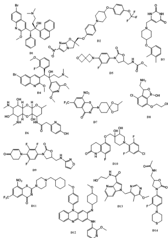
Figure 1: Chemical Structure of Clinical Approved (D1-D2) and Compounds in the Anti-TB Pipeline (D3-D14).
