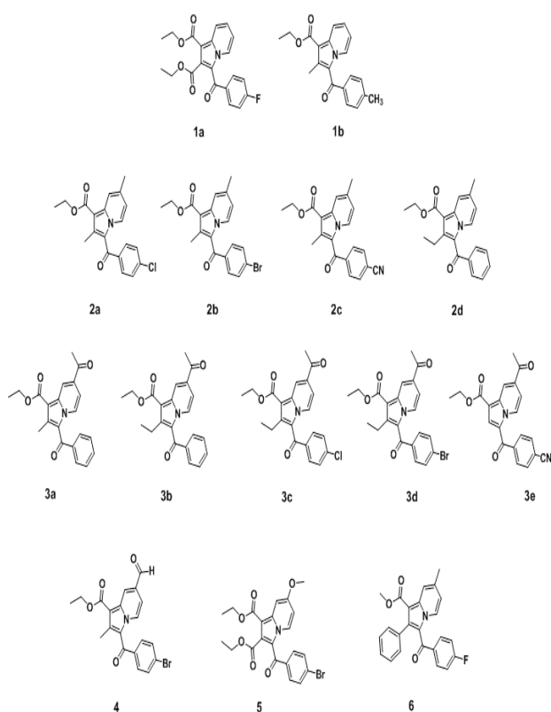
Figure 2: Chemical Structures of Diversely Substituted Indolizine Molecules 1a-b, 2a-d, 3a-e, 4, 5 and 6.
