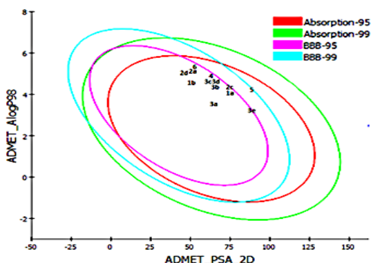
Figure 3: Biplot ADMET_PSA_2D and ADMET_AlogP98 of Investigated Indolizines.
