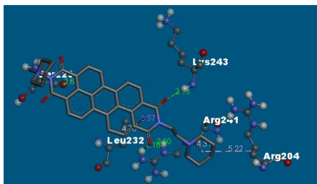
Figure 1: n) Ligand Interactions with the nearby amino acids.
