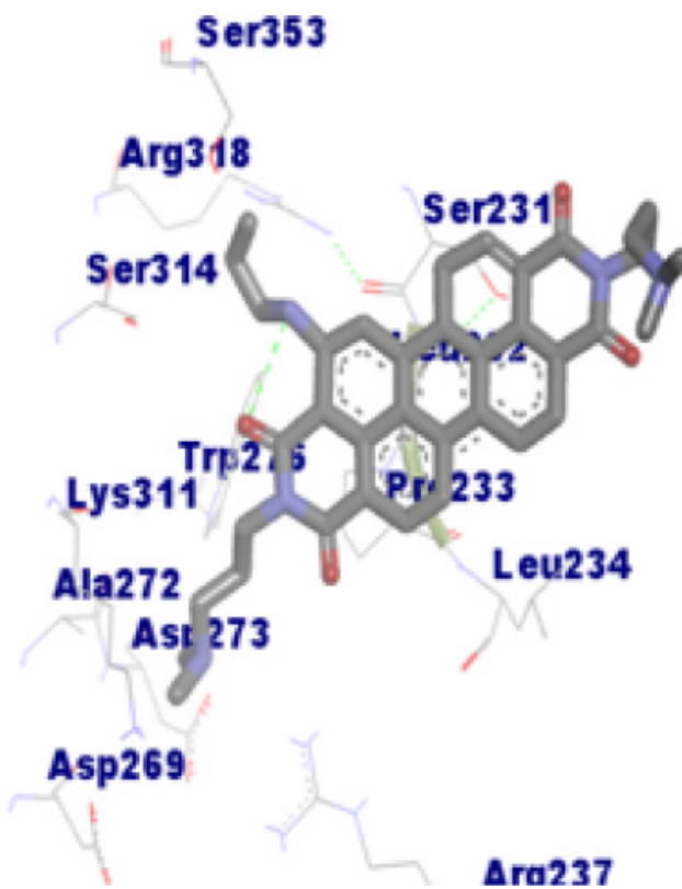
Figure 1: e) Binding Energy: -6.42 kcal/mol
