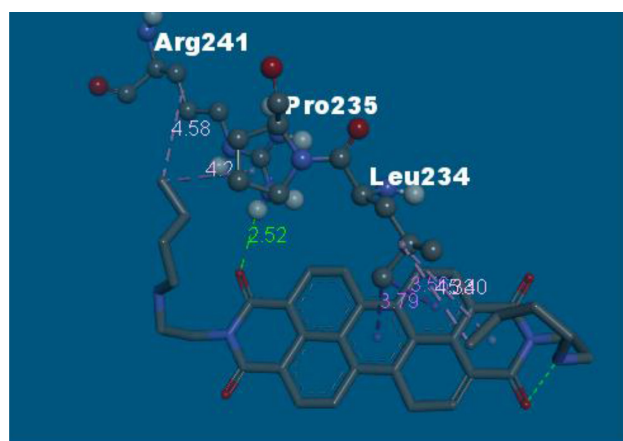
Figure 1: j) Ligand Interactions with the nearby amino acids.
